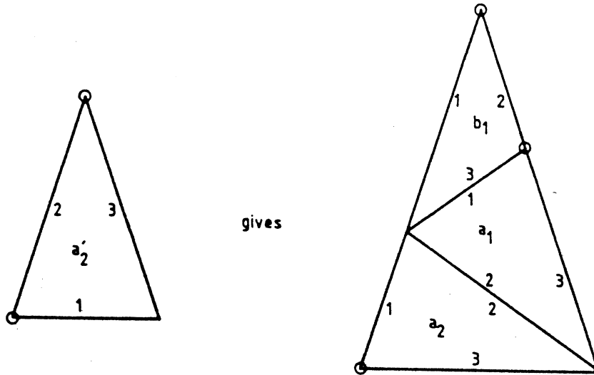
Figure 7 (inflation rule for tile a_2' )
