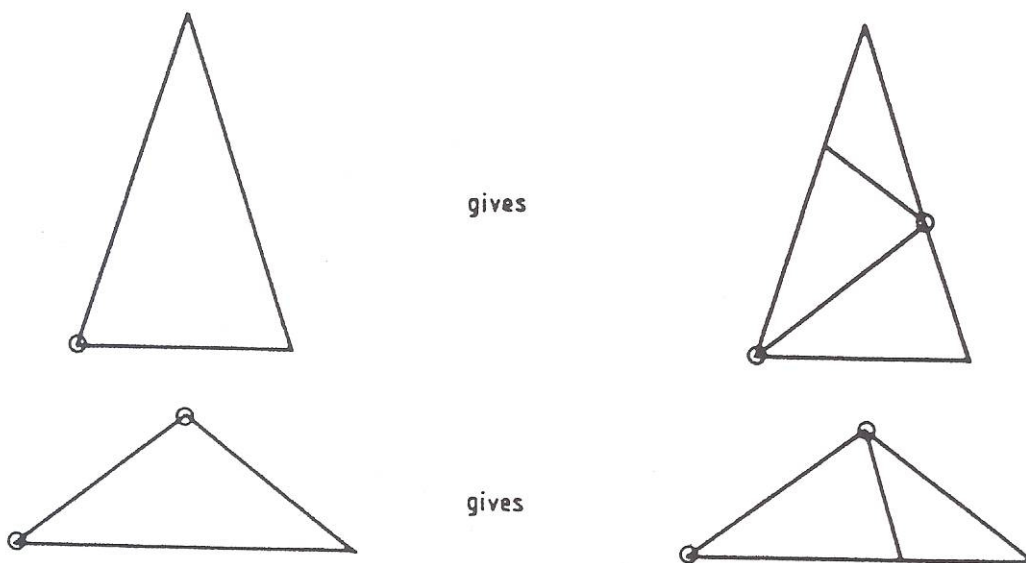
Figure 3 First step of the inflation procedure.
