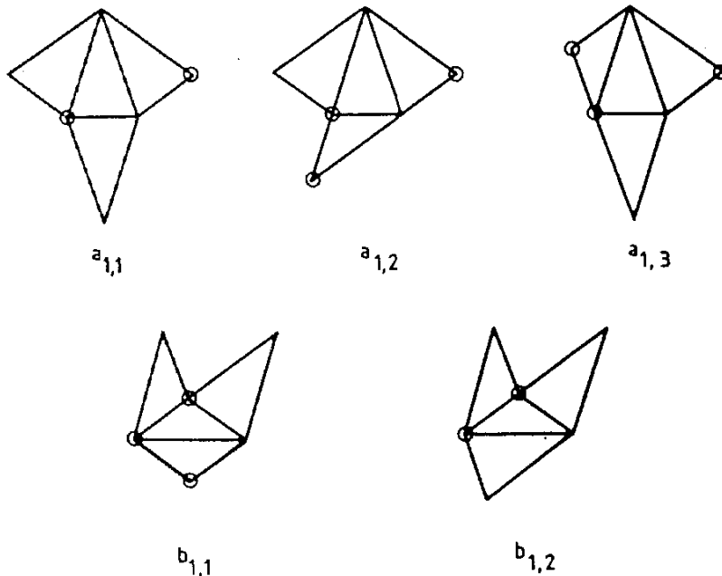
figure 12 five elements of A_1^1 for Penrose tilings.
