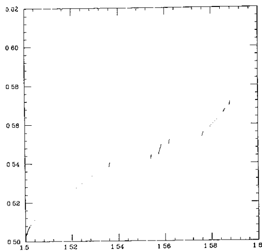
Fig 9 An excerpt of Fig 8 showing the envelope curve at the edge of the center gap ( \lambda = 1.5 ) to be identical with the envelope curve at \lambda = 0
