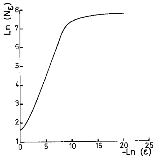
Fig 11 Calculation of the Bouligand-Minkowski dimension d_{BM} . Graph of \log N_\epsilon versus \log(1/\epsilon) for \rho = 0.3 (see text)
