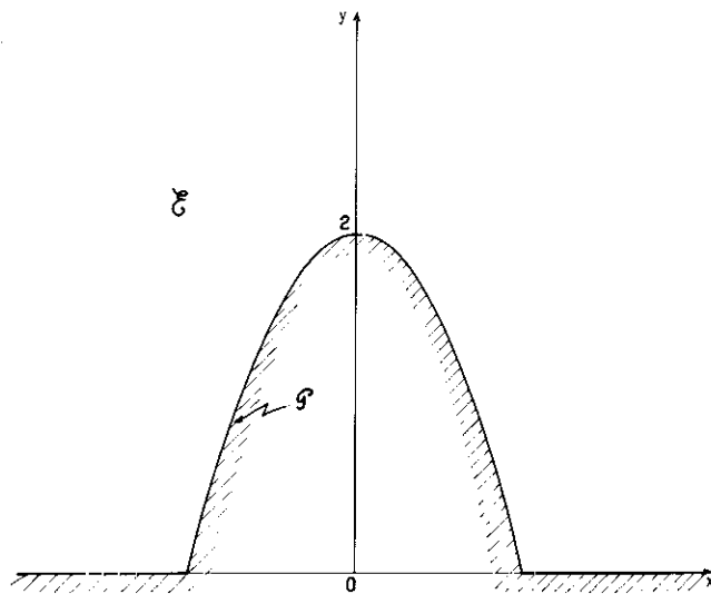
Fig 2 The invariant closed set \mathcal{E} as defined by Eq (35)
