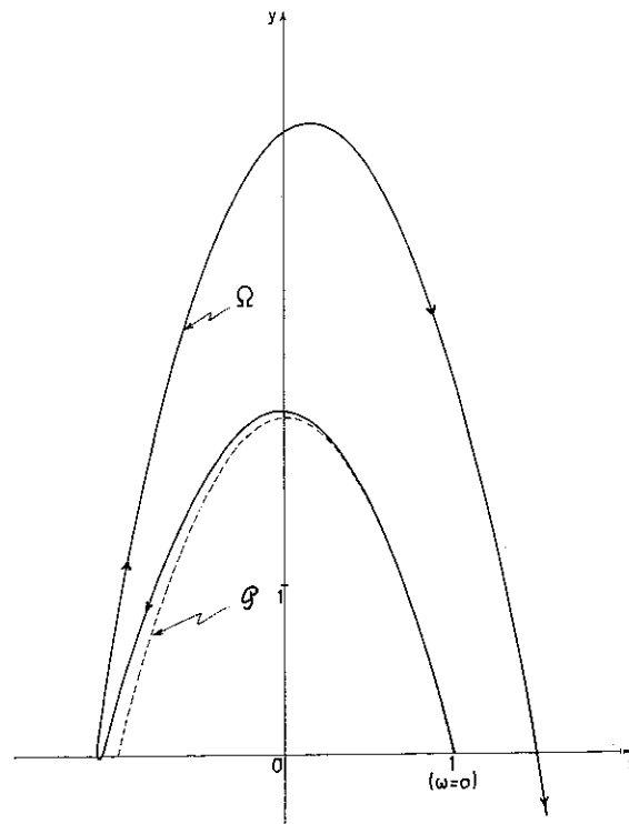
Fig 1 The curve \Omega in the (xy) plane as defined in the text for \rho = 0.6 . The parabola \mathcal{P} has equation y = 2(1 - x^2) .
