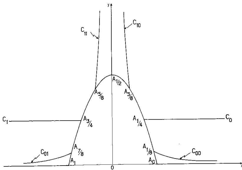
Fig 5 Same as Fig 4, for four iterations of \Phi^{-1}
