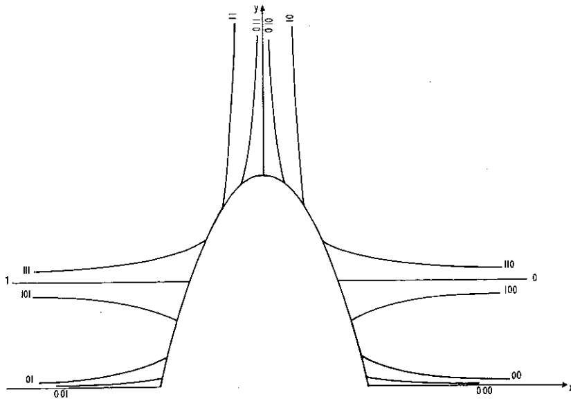
Fig 6 Same as Fig 4, for five iterations of \Phi^{-1} (see text).
